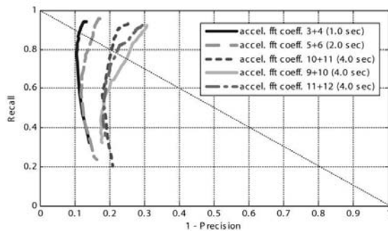
Figure 7: Recognition Results for 'Jogging', using the combinations of (feature; window length) with the highest cluster precision for this activity.
