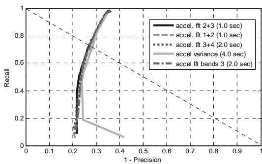
Figure 6: Recognition Results for 'Riding Bus', using the combinations of (feature; window length) with the highest cluster precision for this activity.
